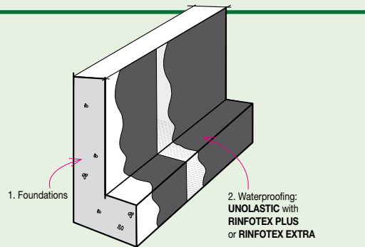
Protect the waterproofing with PROTEFON TEX or EPS panels
