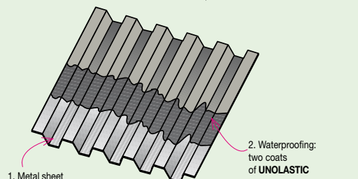
UNOLASTIC can be painted over with WHITE REFLEX reflecting paint or ELASTOLIQUID S paint
