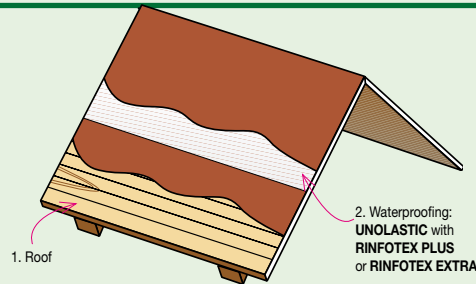
Wooden and concrete roofs
